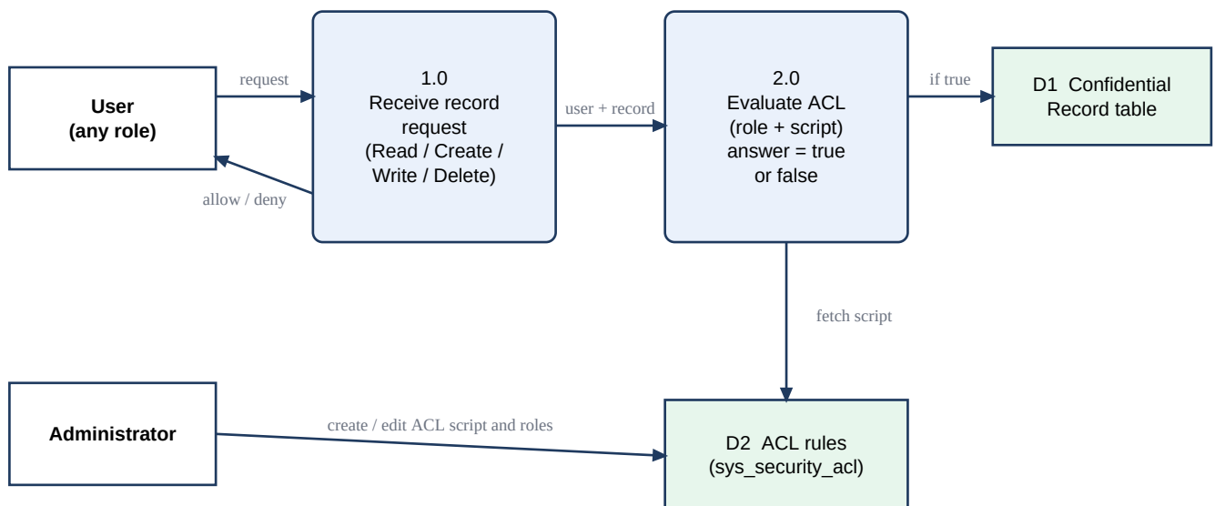
Figure 1: Data flow of a record request through the script-controlled ACL
